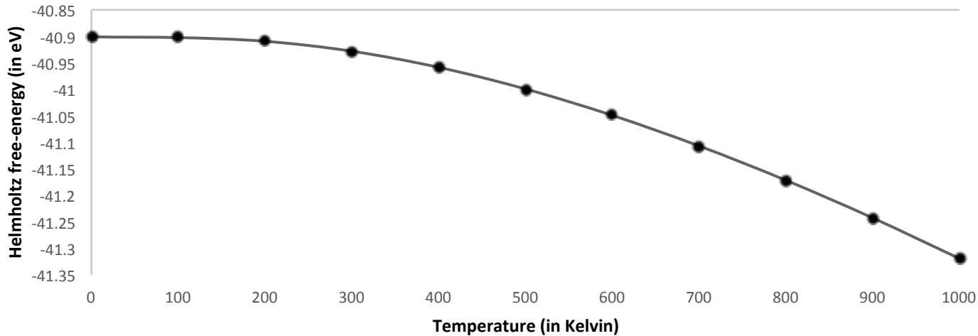
Helmholtz free-energy against Temperature
