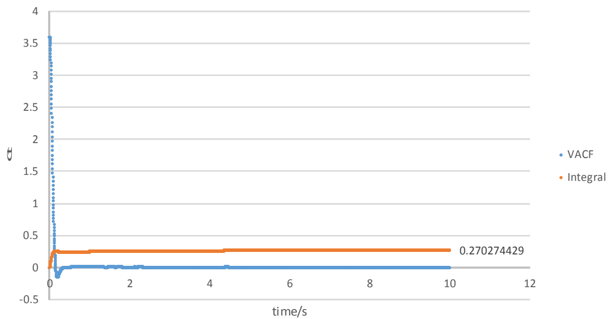
Graph of VACF and integral for a million atom simulation for a liquid
