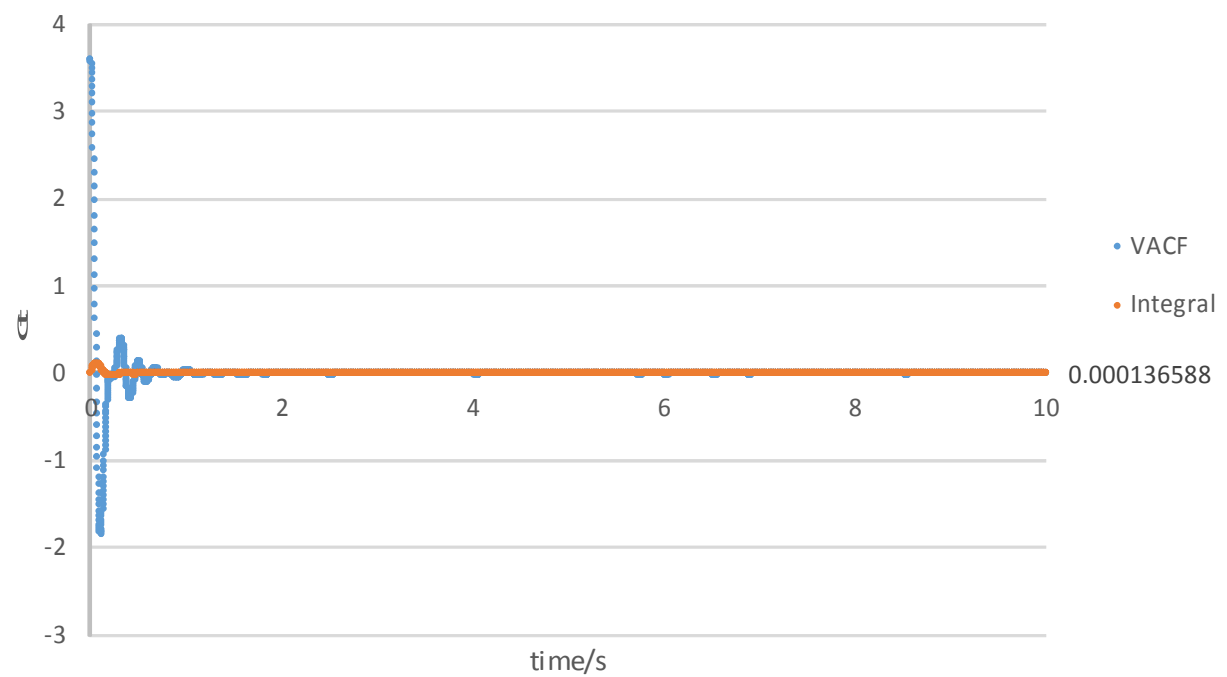
graph of VACF and integral of a million atom simulation for a solid
