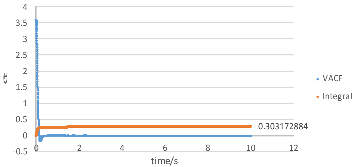
Graph of VACF and integral for a million atom simulation for a liquid
