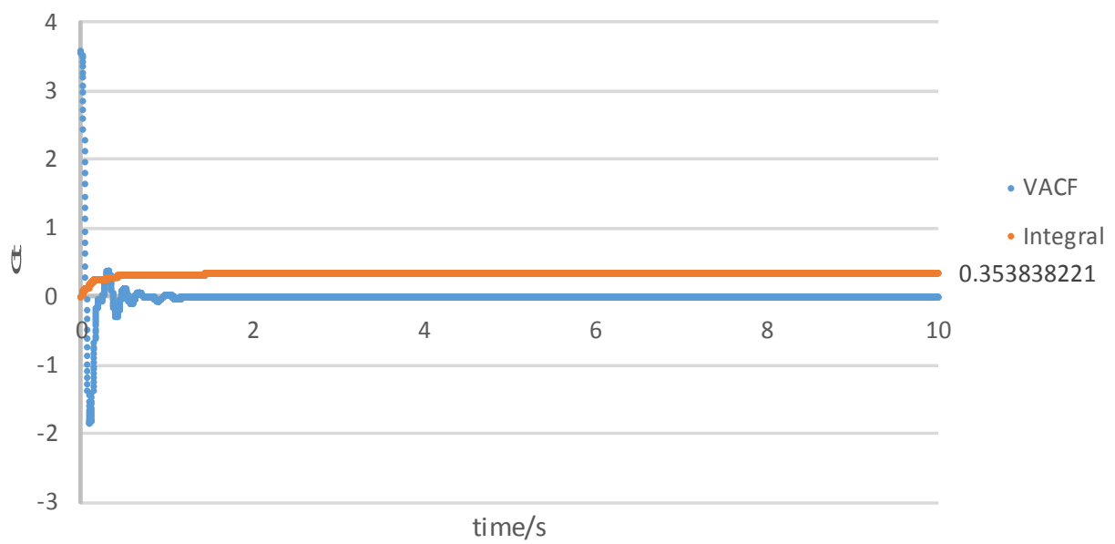
graph of VACF and integral of a million atom simulation for a solid
