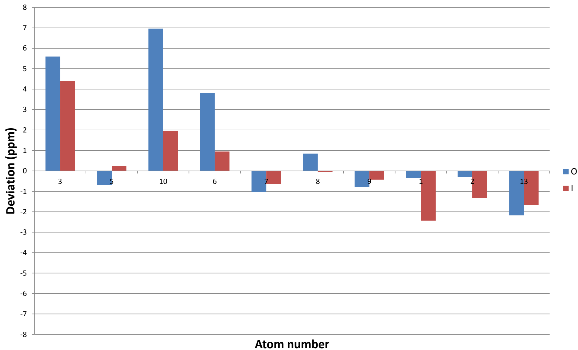
Deviations of calculated shifts for O and I from shifts of natural product
