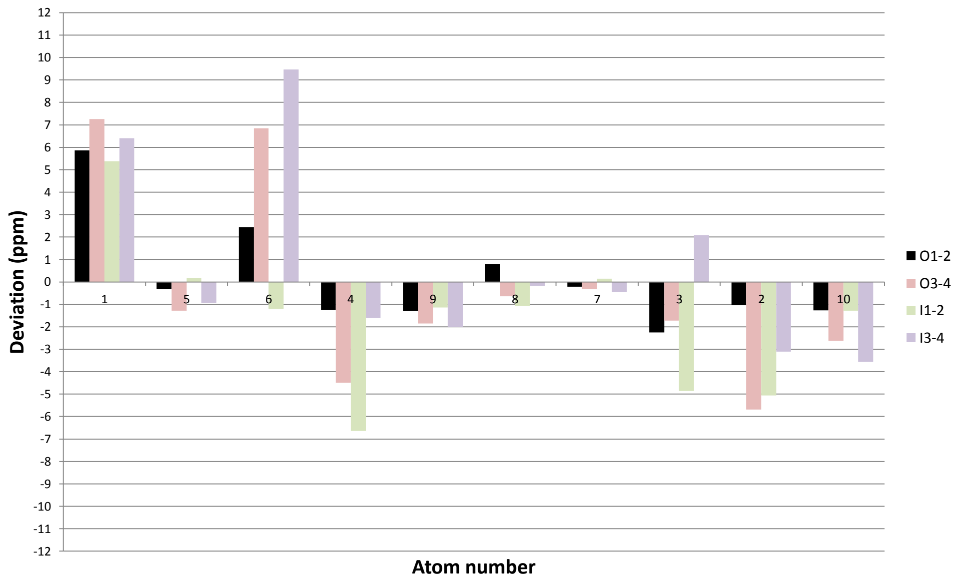
Deviation of calculated shifts from O major shifts
