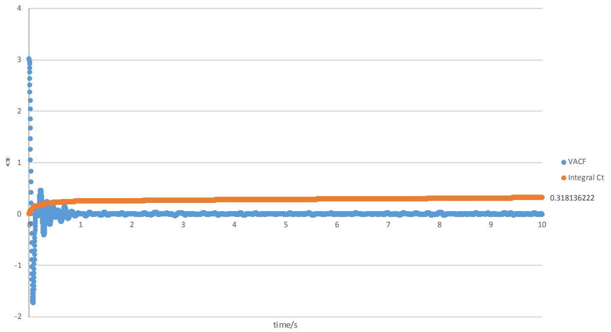
Graph of VACF and its integral for a solid
