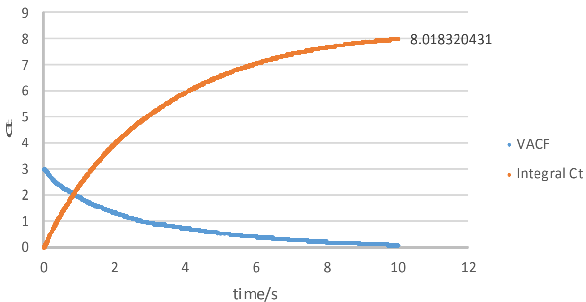
Graph of VACF and its integral for a gas
