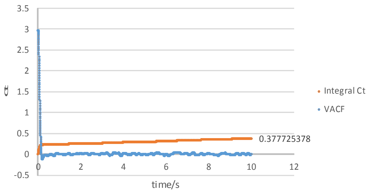
graph of VACF and its integral for a liquid
