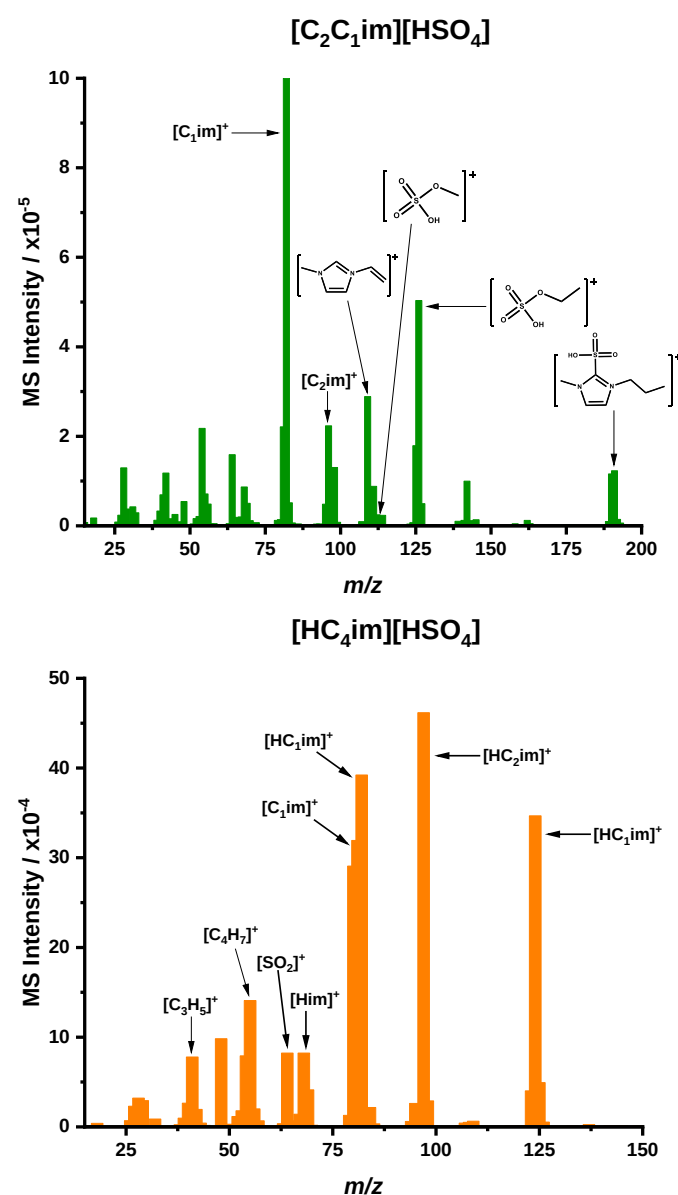
Figure 10a Histograms for vapour phase components of (6) [\text{C}_2\text{C}_1\text{im}][\text{HSO}_4] at T_{\text{onset}} 368.6 °C (green) and (5a) [\text{HC}_4\text{im}][\text{HSO}_4] at T_{\text{onset}} 342.5 °C (orange) using DIP-MS in the positive mode.
