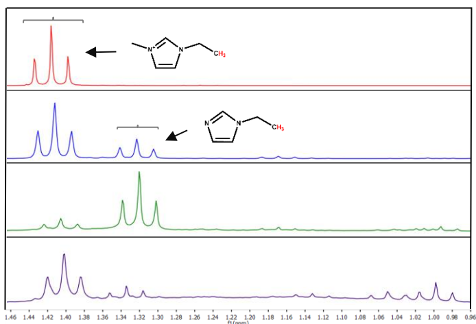
Figure 11b Expanded regions of the ^1\text{H} NMR spectrum of [\text{C}_2\text{C}_1\text{im}][\text{OAc}] after heating at 180^\circ\text{C} for 0, 1, 24 and 48 hours; Peaks for the formation of decomposition products such as [\text{C}_2\text{im}]^+ .
