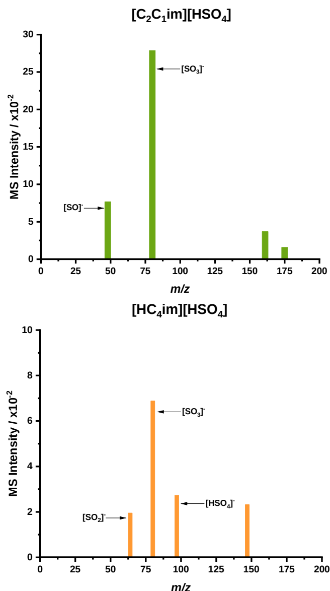
Figure 10b Histograms for vapour phase components of (6) [\text{C}_2\text{C}_1\text{im}][\text{HSO}_4] at T_{\text{onset}} 368.6 °C (green) and (5a) [\text{HC}_4\text{im}][\text{HSO}_4] at T_{\text{onset}} 342.5 °C (orange) using DIP-MS in the negative mode.
