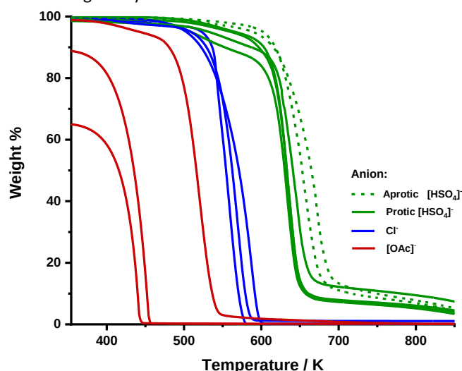
Figure 5 TGA thermographs for several imidazolium [HSO 4 ] - based PILs (solid green) AIL (dashed green); Aprotic imidazolium and ammonium chlorides (blue); Aprotic and protic imidazolium and protic ammonium acetate ILs (red)
