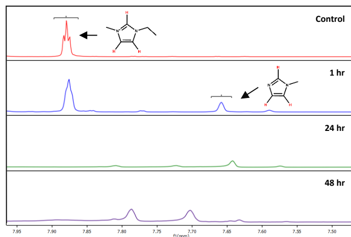
Figure 11a Expanded regions of the ^1\text{H} NMR spectrum of [\text{C}_2\text{C}_1\text{im}][\text{OAc}] after heating at 180 °C for 0, 1, 24 and 48 hours; Peaks shown in the aromatic region for the imidazole.
