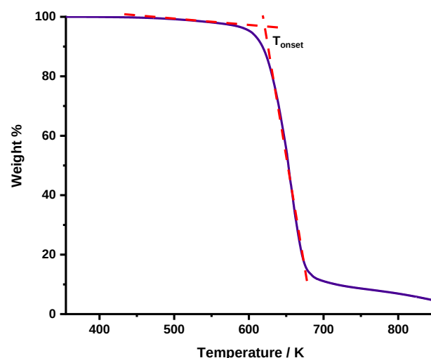
Figure 3 Typical TGA thermograph showing tangents used to obtain T_{onset}
