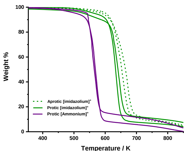
Figure 6 TGA thermographs of hydrogen sulphate ILs using either imidazolium cations: [C 2 C 1 im] + (6), [C 4 C 1 im] + (3) (dashed green) and [HC 1 im] + (4), [HC 4 im] + (5a) (solid green) or ammonium cations; [N 2220 ] + (2), [N 4110 ] + (1) (purple).
