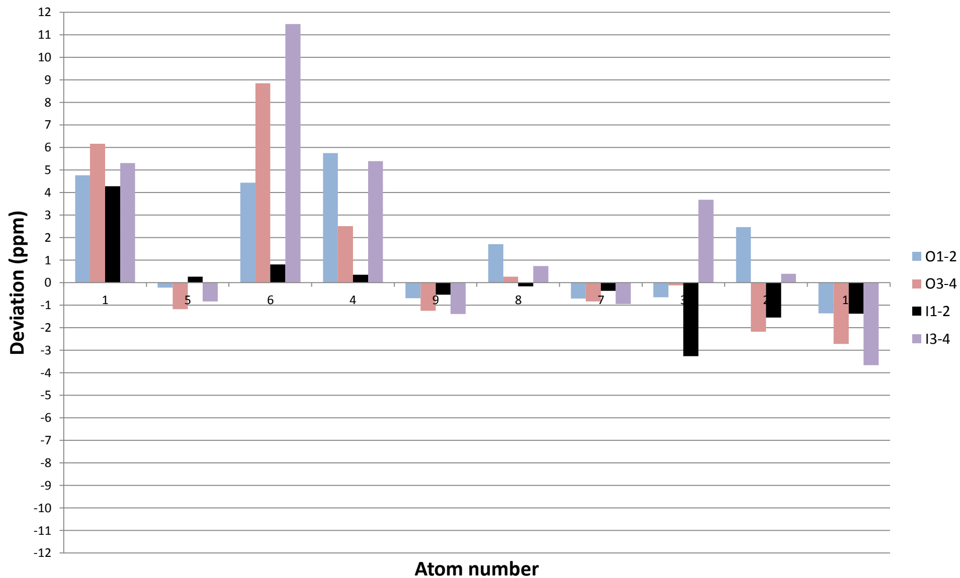
Deviation of calculated shifts from "2' major" shifts
