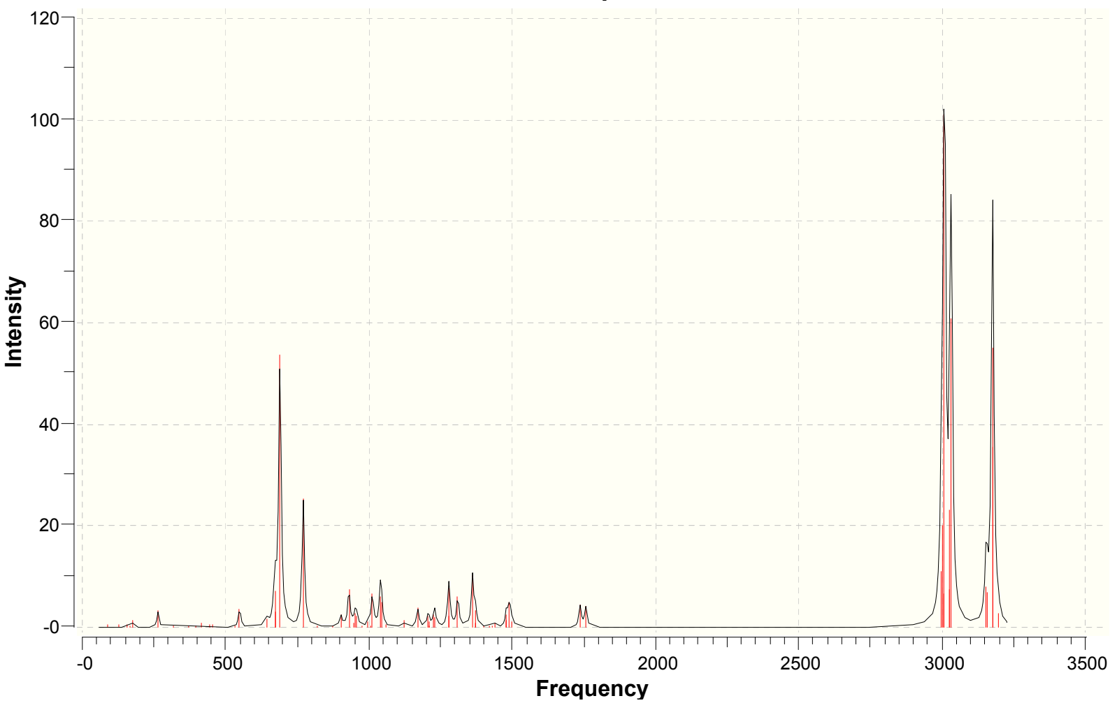
Infrared Spectrum
