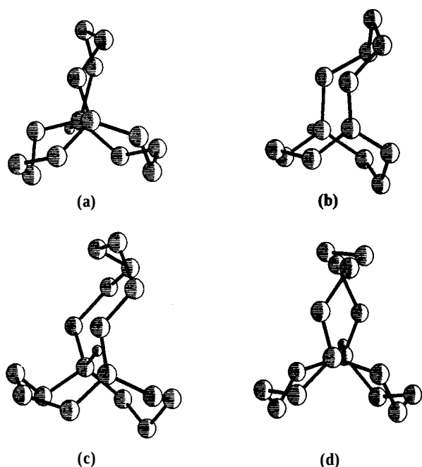
Figure 1. Examples of global minima found by GMMX. (a) out -bicyclo[4.4.4]tetradec-1-ene. (b) out - bicyclo[5.3.3]tridec-1-ene. (c) in - bicyclo[7.4.4]heptadec-1-ene. (d) in - bicyclo[6.4.4]hexadec-1-ene. Hydrogens except at the bridgehead position are omitted for clarity.
