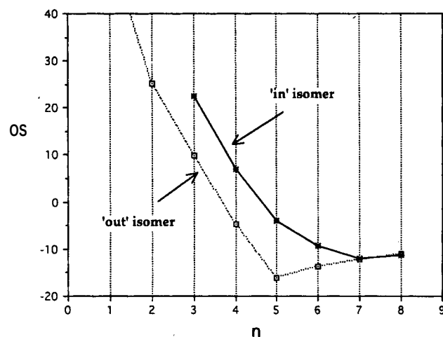
Figure 5. Olefin strain (OS, in kcal/mol) vs. chain size (n) for 'in' and 'out' bicyclo[n.3.3] bridgehead olefins.
