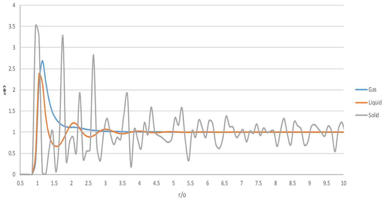
radial distribution functions of three states of matter
