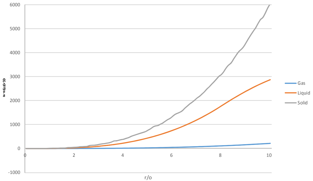
integral radial distribution functions for three states of matter
