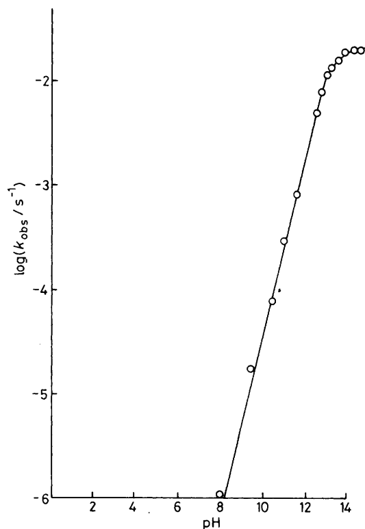
Figure. pH-rate profile for the cyclisation of (11a) in 1:1 aqueous acetonitrile at 39 °C and ionic strength 0.2M (KCl). Open circles are experimental points, the curve is calculated (for constants see Tables 1 and 2), assuming that only the phenolate anion is reactive
