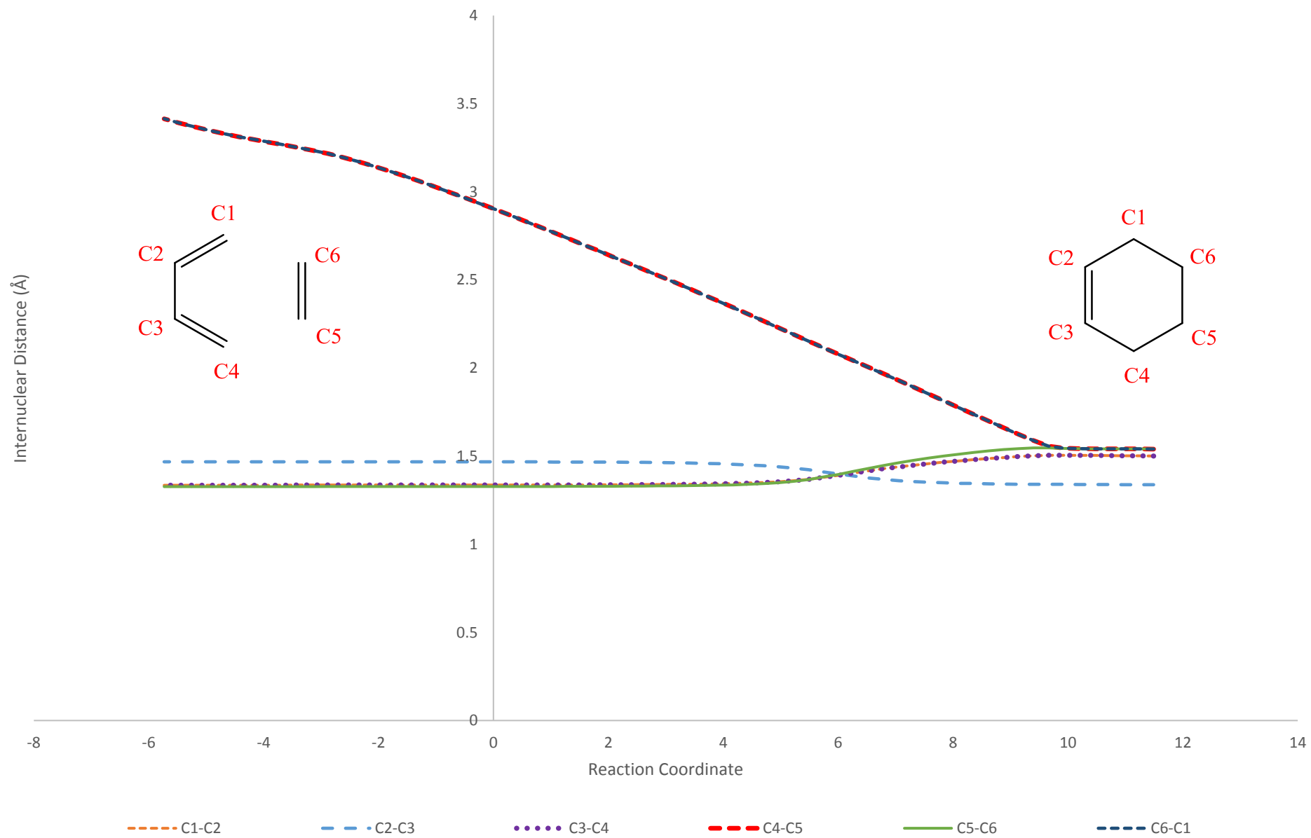
Internuclear distances for the reaction of butadiene with ethylene
